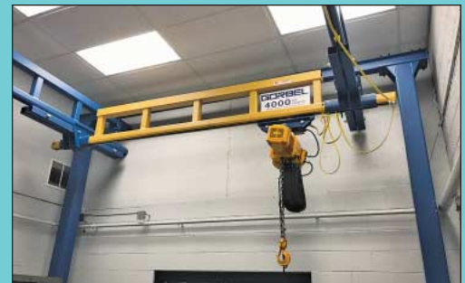
2 Ton x 12' (Approx.) Span x 15' (Approx.) Long Gorbelt Free Standing Overhead Bridge Crane System
